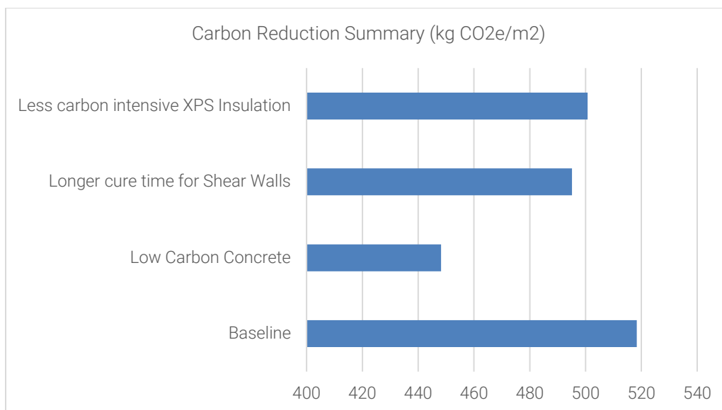
Figure 19– Embodied Carbon Reduction Summary Graph
