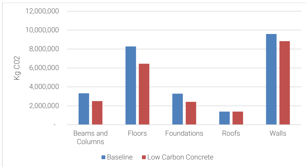
Figure 18 – Low Carbon Concrete – 30-40% SCM and GUL
